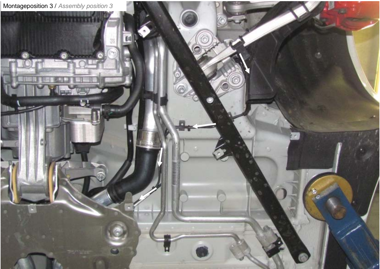
Montageposition 3 / Assembly position 3
